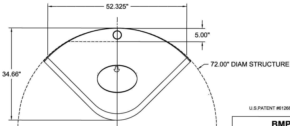
PLAN
