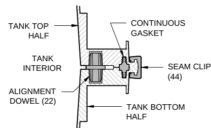
S MID-HEIGHT SEAM SECTION DETAIL
