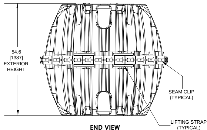
END VIEW
