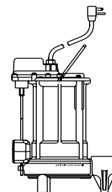
Model 257 VMF VMF switch, magnetically operated vertical float – operates in a 10" diameter sump.
