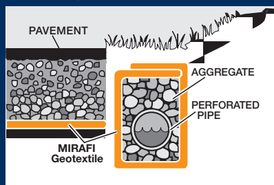
Cut-off/Inceptor Drain Along a Roadway Or Another Critical Struction
