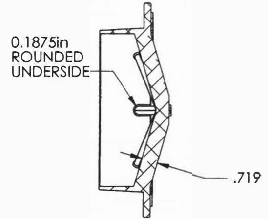
SECTION B-B
